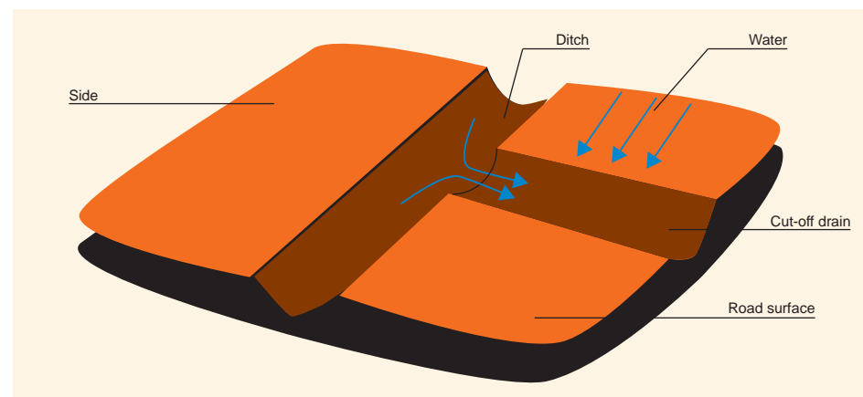
Illustration: How to make cut-off drains
