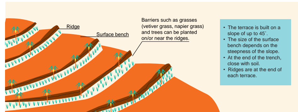
Illustration: How to build bench terraces
