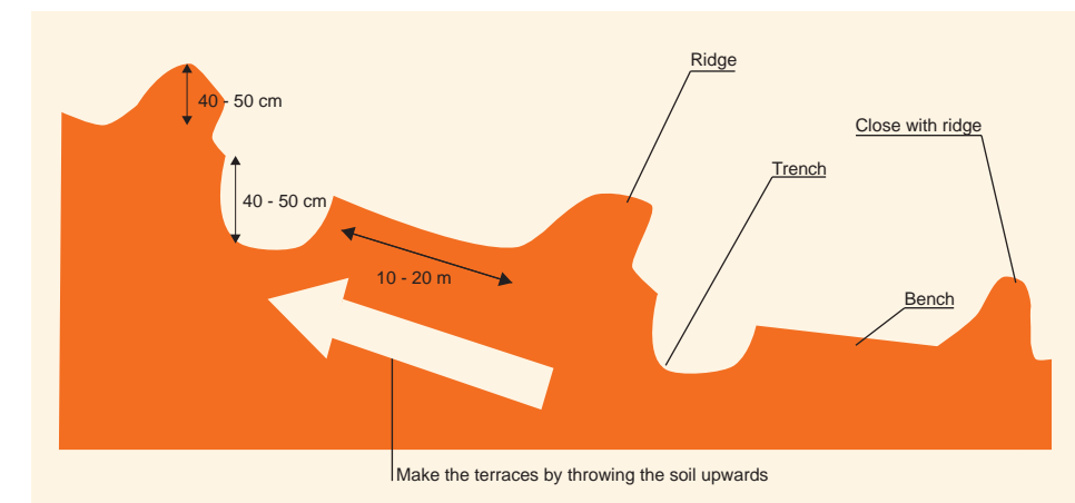
Illustration: How to build fanya juu terraces
