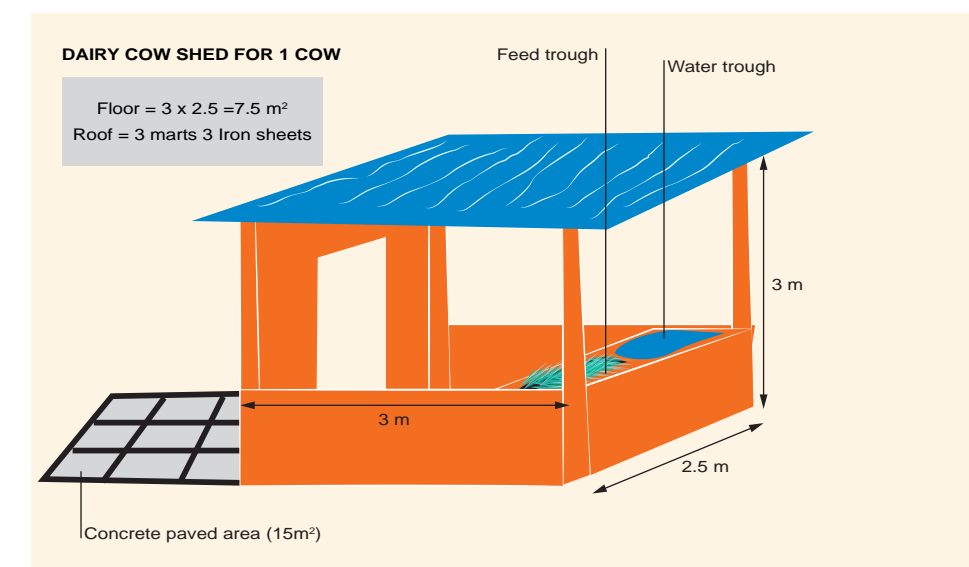
Illustration: Housing for cows
