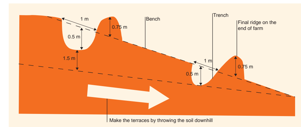
Illustration: How to build fanya chini terraces
