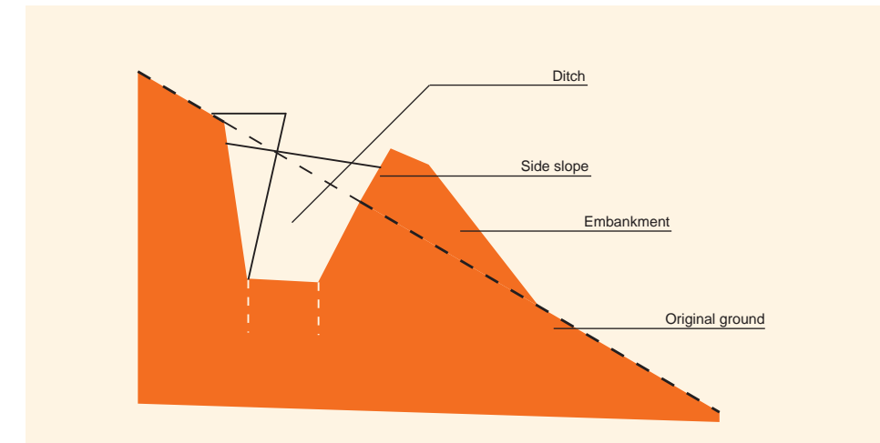
Illustration: How to make a diversion ditch
