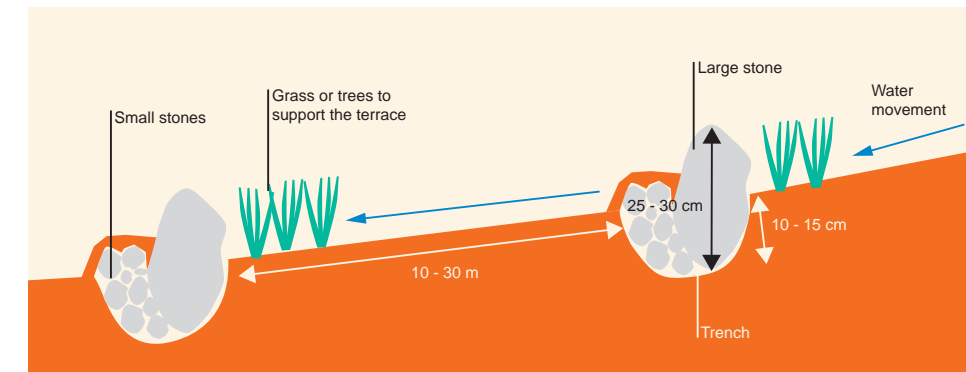
Illustration: How to build stone terraces
