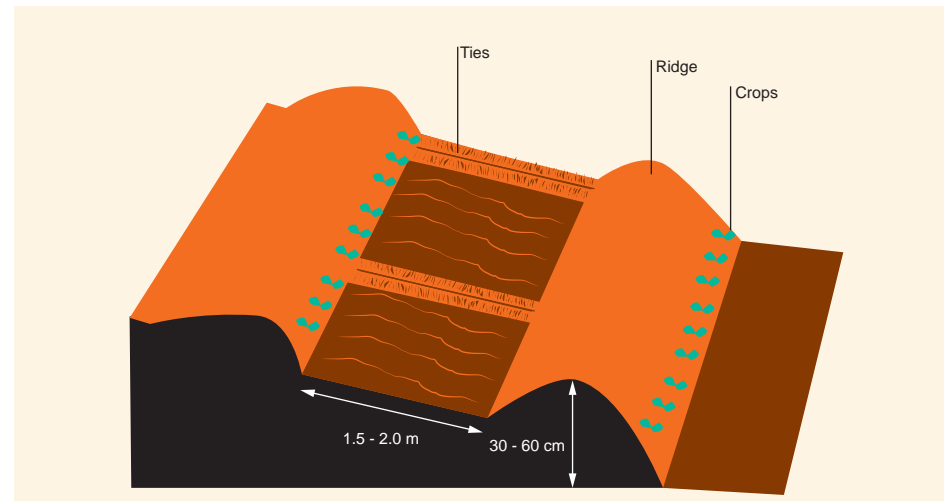
Illustration: How to make tied ridges
