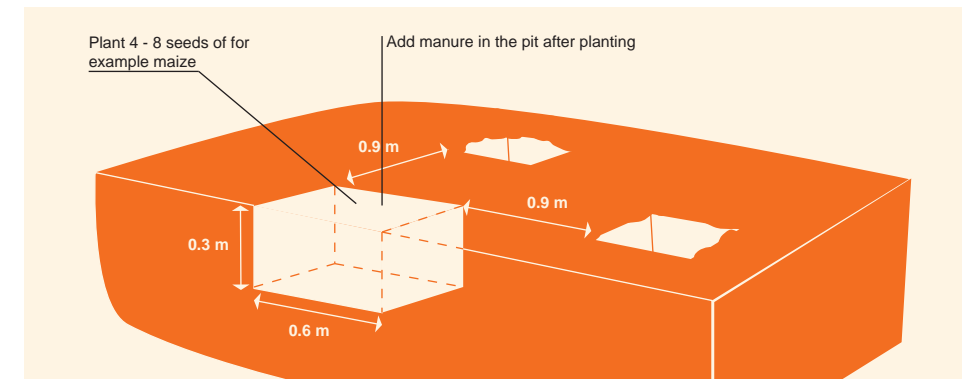
Illustration: How to make zai pit
