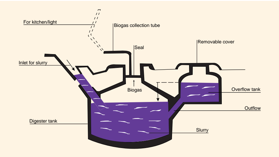
Illustration: Biogas digester
