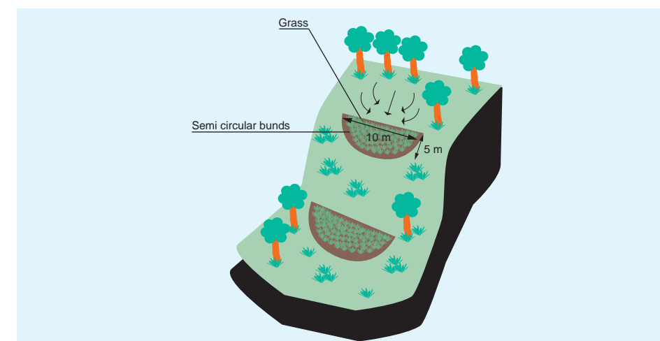
Illustration: How to make semi-circular bunds
