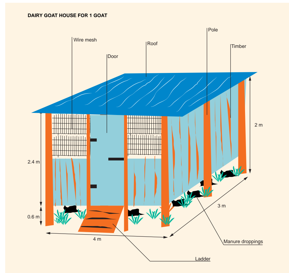
Illustration: Housing for dairy goats
