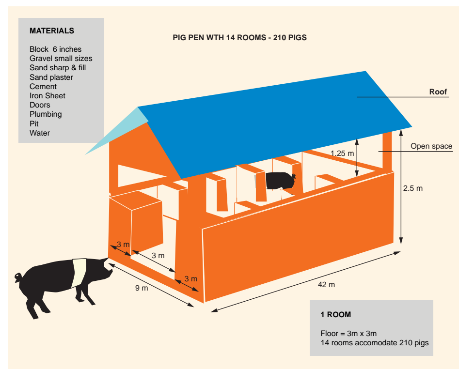
Illustration: Housing for pigs
